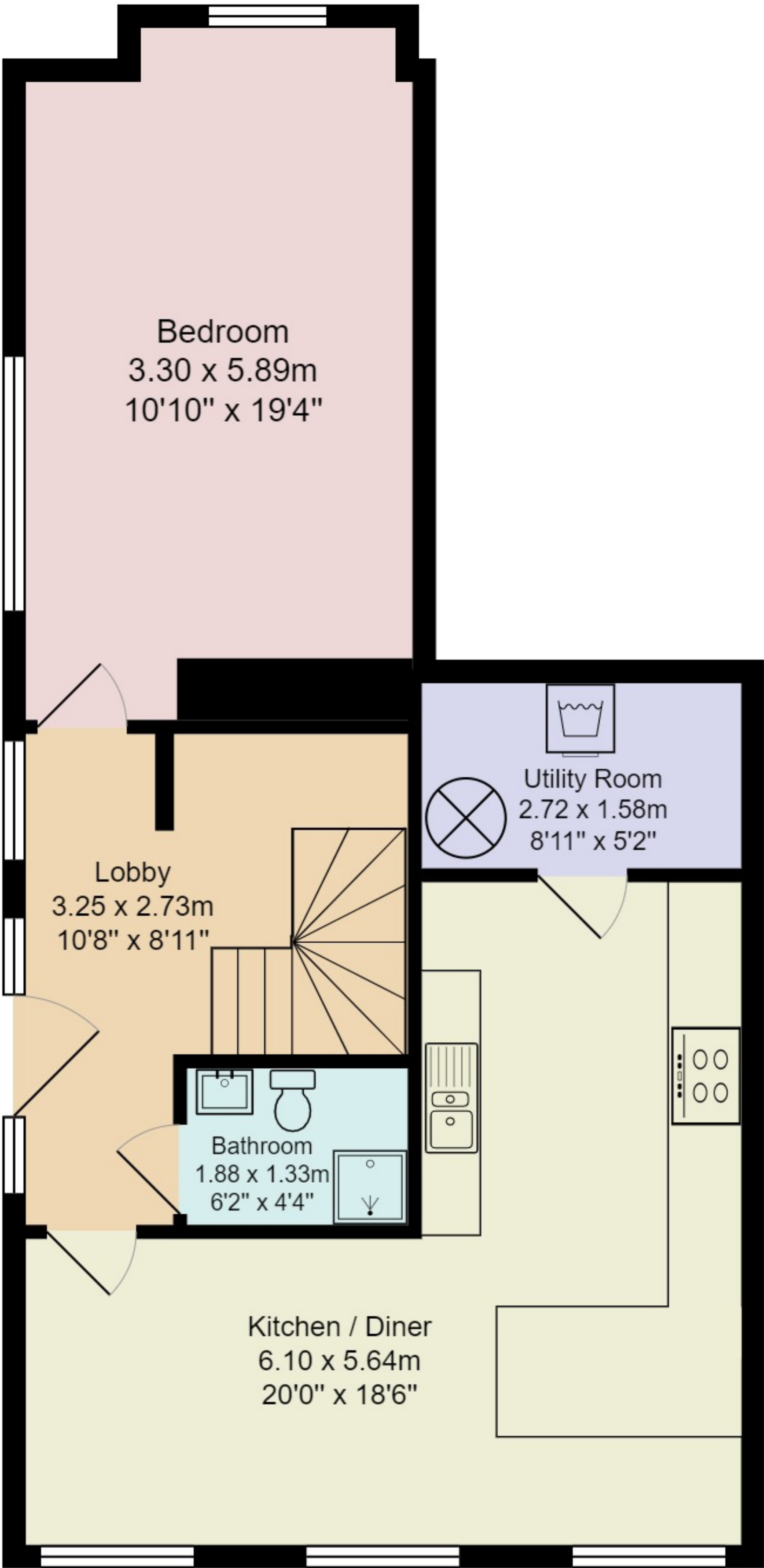
Ground Floor
